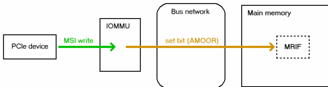
Figure 8.2: Recording an incoming MSI into a memory-resident interrupt file (MRIF) instead of sending it to a guest interrupt file as in Figure 8.1.
