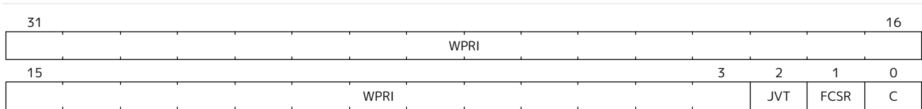
Figure 37. Supervisor State Enable O Register ( ssstateen0 )
