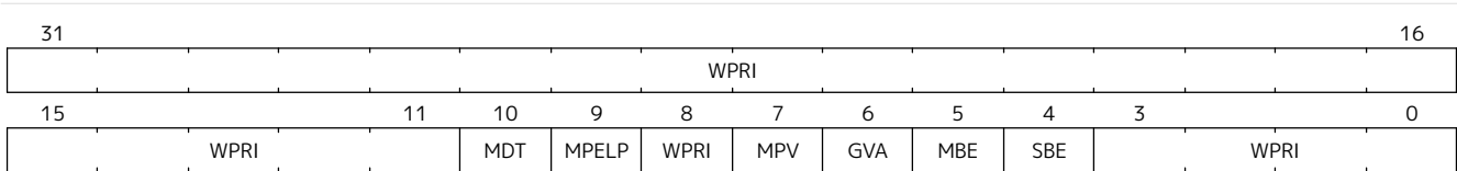
Figure 9. Additional machine-mode status ( mstatus ) register for RV32.
